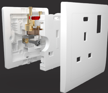
Socket Assembly
